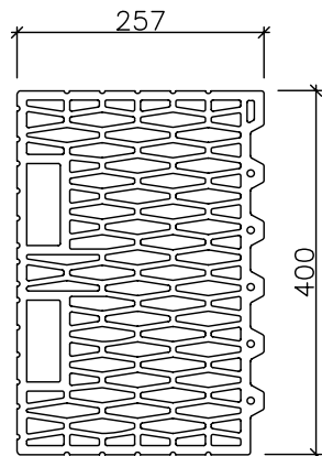
POROTHERM 40 K
