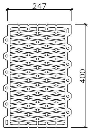
POROTHERM 40 P+D
