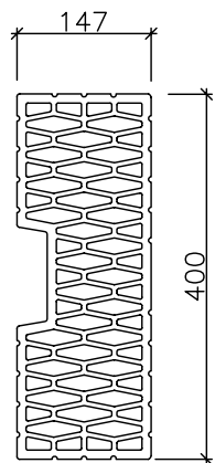
POROTHERM 40 R
