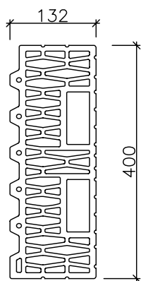
POROTHERM 40 1/2 K
