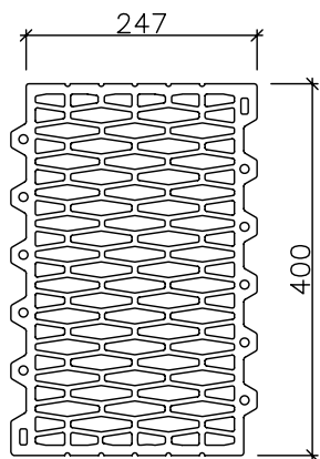
POROTHERM 40 CB
