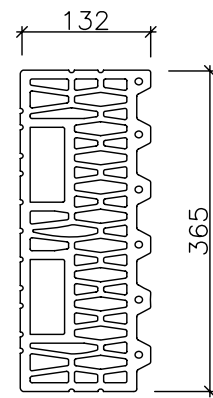
POROTHERM 36,5 1/2 K
