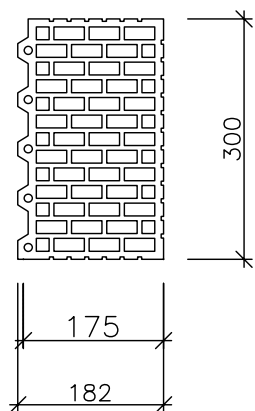
POROTHERM 30 R P+D (CB)
